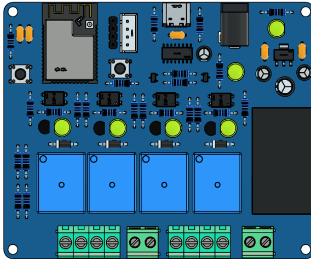
Figure 3: Custom 4-Channel PCB Layout Component Placement
